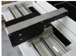
Telescopic pusher.
